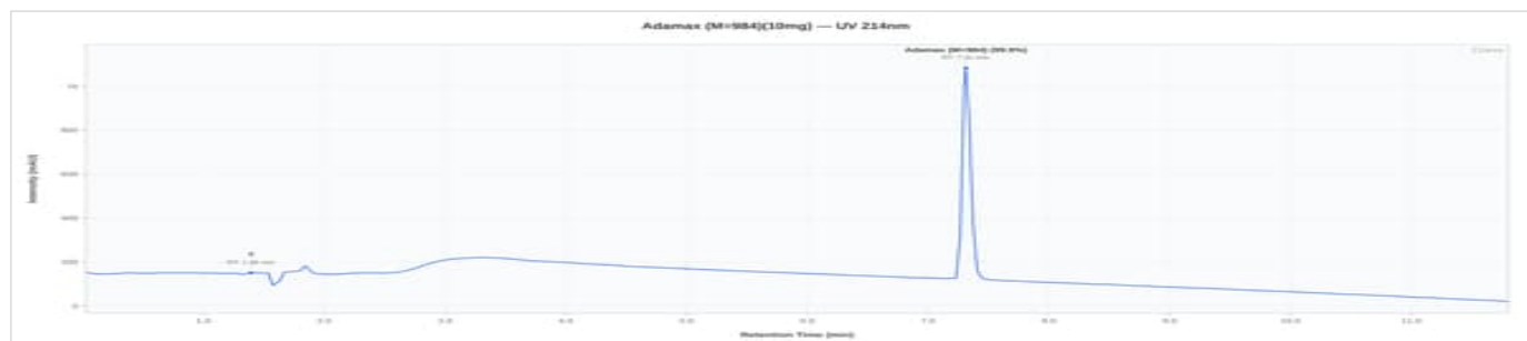
Adamax 10mg - 0726: UV Chromatogram
